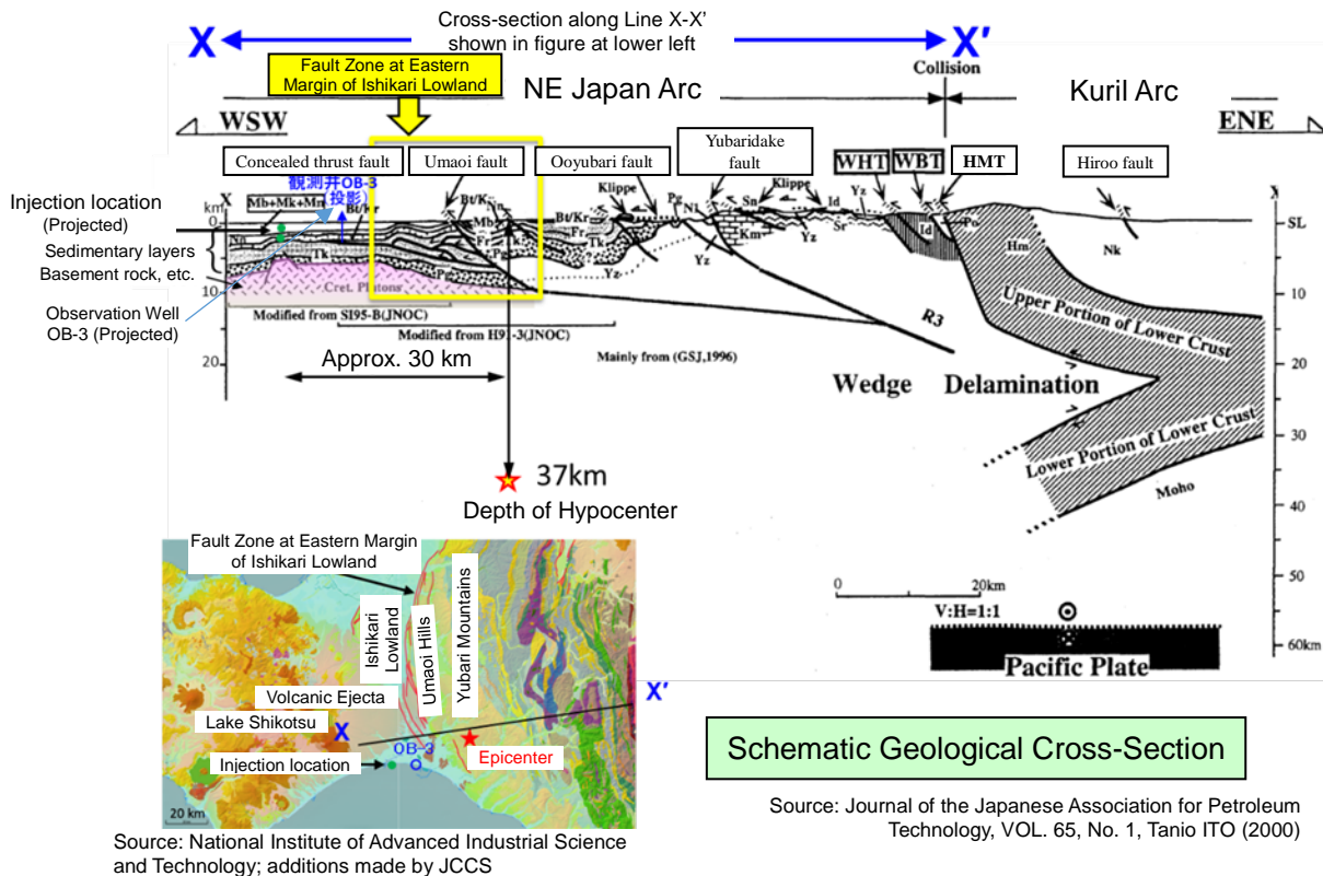
Figure 6: Hypocenter of Hokkaido Eastern Iburi Earthquake and schematic geological cross-section
